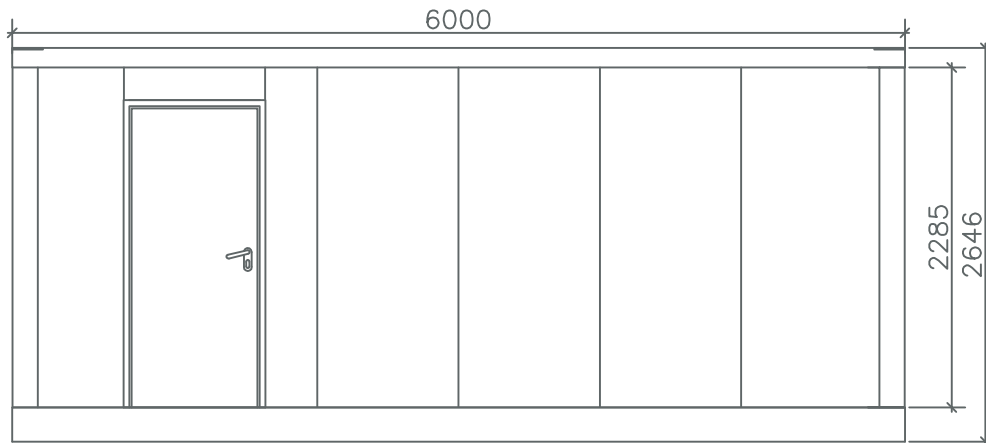
ALZADO PRINCIPAL
