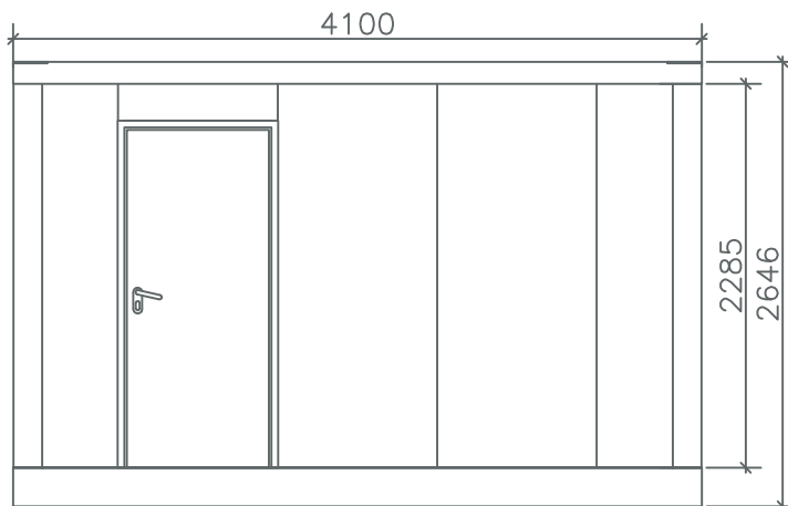
ALZADO PRINCIPAL
