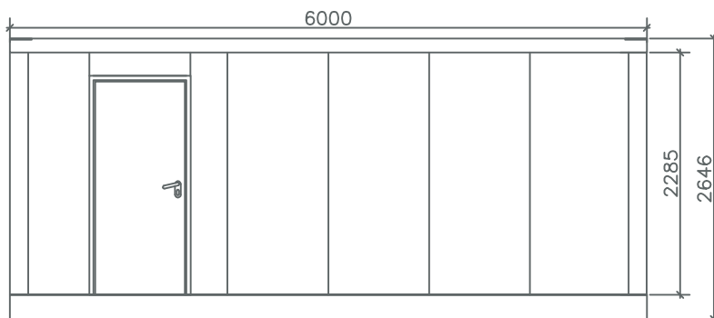
ALZADO PRINCIPAL
